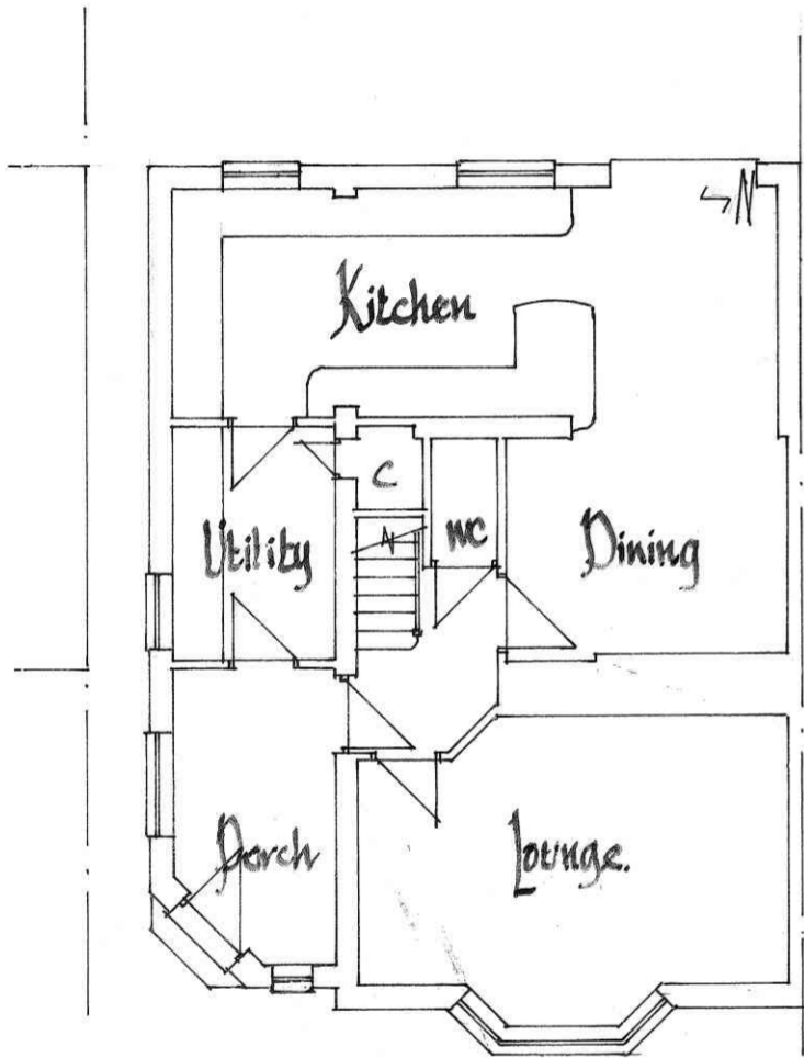
Proposed Ground
